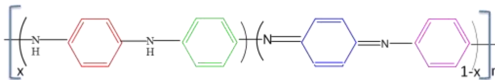
Figure 1 General formula for different forms of polyaniline base
