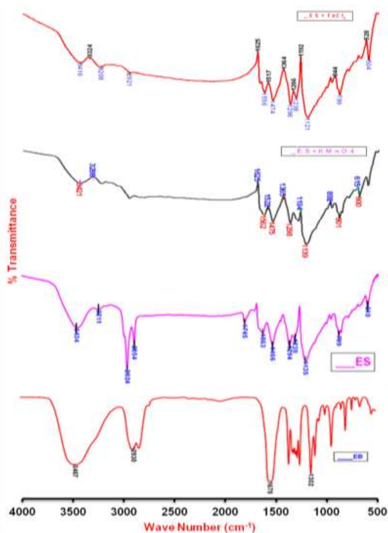
Figure 6 FTIR of Undoped, primary doped PANI- HCl (ES), secondary doped with \text{FeCl}_3 and \text{KMnO}_4
